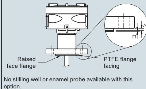
Flange facing (raised face)
