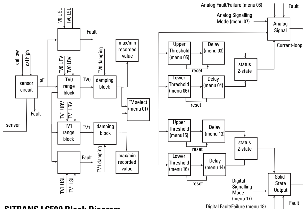
SITRANS LC500 Block Diagram
